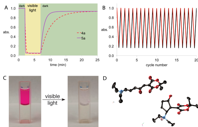
Figure 3. (A) In situ kinetic plot of the switching cycle of 4a and 5a in PhMe, monitored at \lambda_{\max} of 545 and 570 nm, respectively. (B) Multiple photoswitching cycles of 5a in PhMe (0.16 mM), alternative irradiation at 570 nm (red) and dark (black). (C) Photographs illustrating the concomitant photoswitching and phase transfer of 4a upon irradiation with visible light. (D) ORTEP drawings of 4a (top) and 4b (bottom) (50% probability ellipsoids, hydrogen atoms omitted for clarity).
