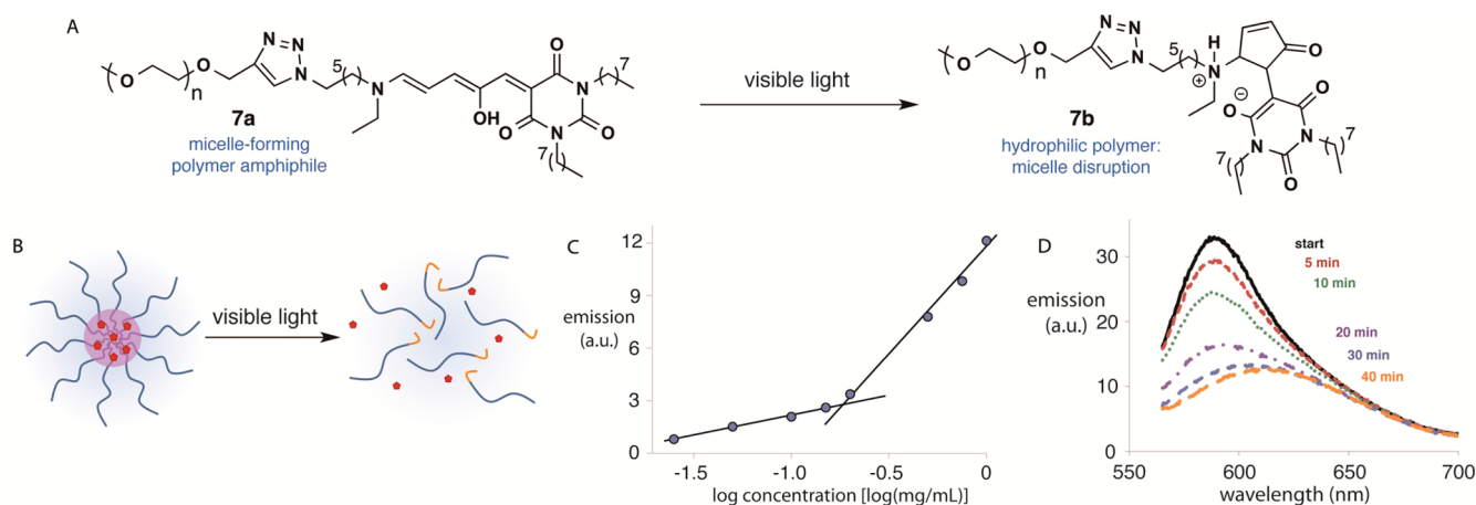
Figure 4. (A) Photoswitching of micelle-forming polymer amphiphile. (B) Schematic of micelle formation and hydrophobic cargo encapsulation by functional amphiphile 7a and micelle disruption and cargo release on visible light irradiation. (C) Fluorescence intensity ( E_m at 588 nm) vs log concentration (mg/mL) of 7a. (D) Fluorescence emission spectra of Nile Red in 0.50 mg/mL 7a in water at various times of visible light irradiation.
