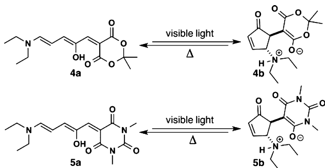
Scheme 2. Photoswitching and Thermal Reversion of Trienes 4a and 5a to Cyclopentenones 4b and 5b
